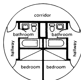
Nassauer Hof Hotel, Wiesbaden 6 Typical hotel layout
